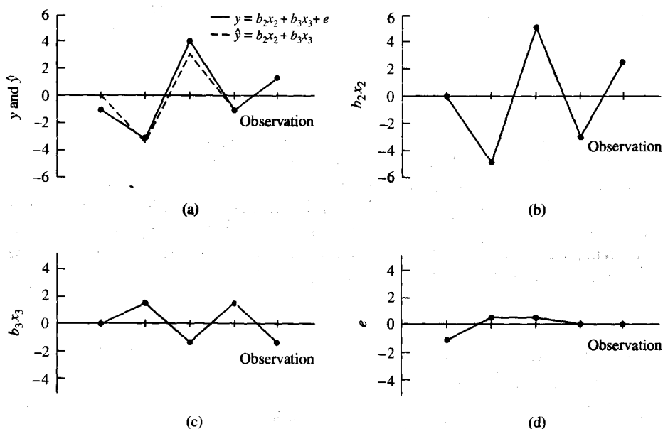
FIGURE 3.1 Tinbergen Diagram for Example 3.3
