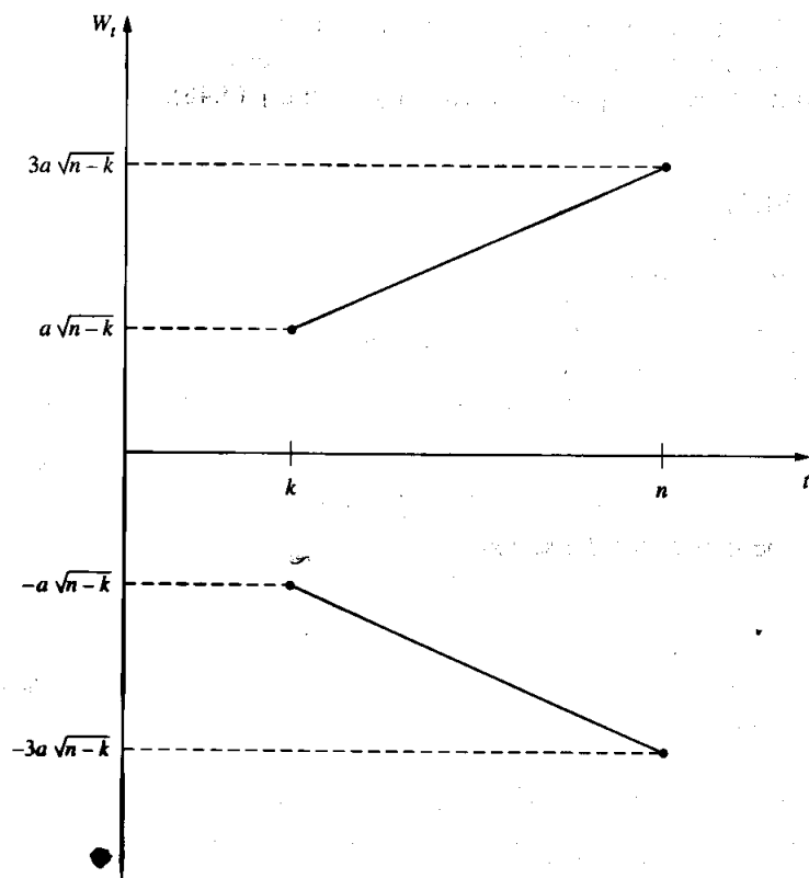
FIGURE 4.1 CUSUM plot.
