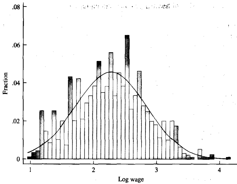
FIGURE 11.7 Histogram with 50 bins.
