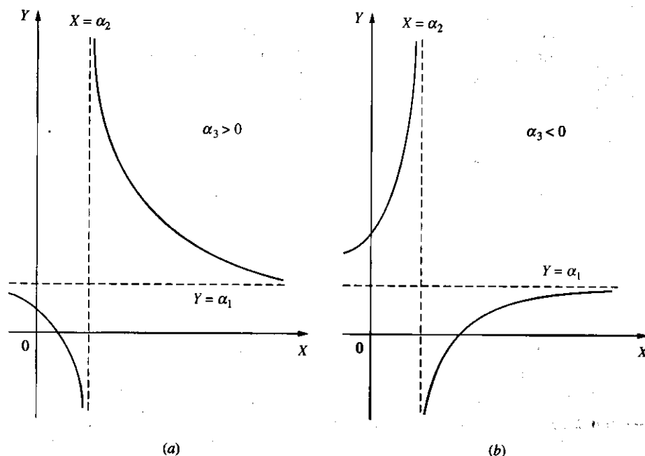
FIGURE 2.3 Rectangular hyperbola.
