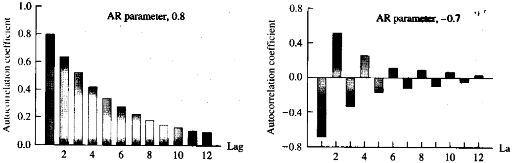
FIGURE 7.1 Correlograms for stationary AR(1) series.
