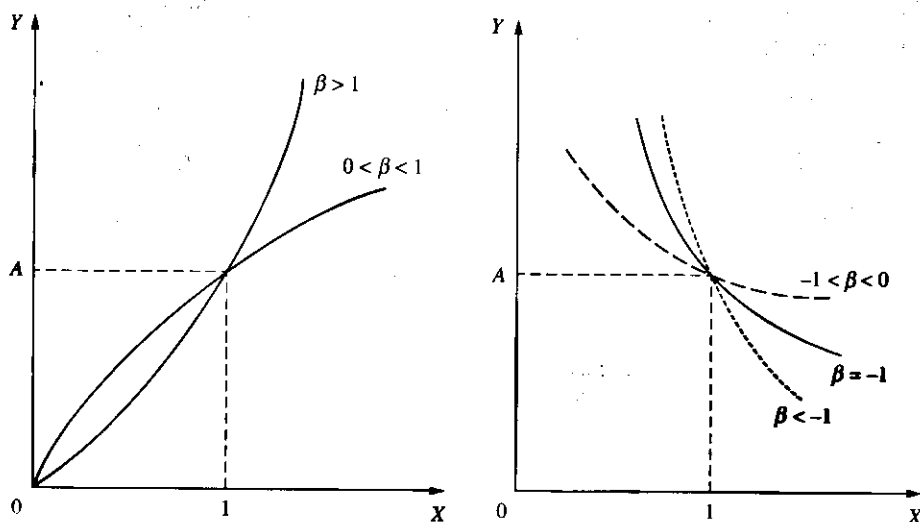
FIGURE 2.1 Y = AX^\beta .
